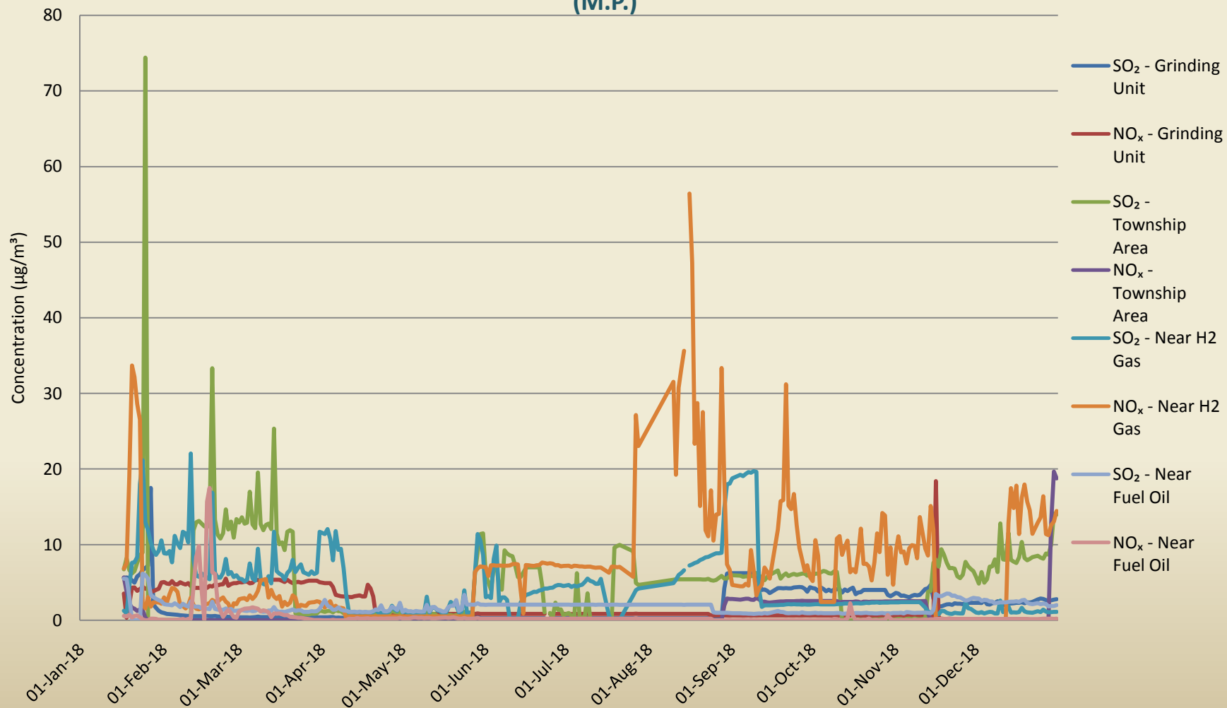
Annual Ambient Trend of Gaseous in M/s. Jaypee Power Ventures Limited, Dist. Singrauli (M.P.)
